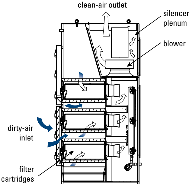
NORMAL OPERATION
