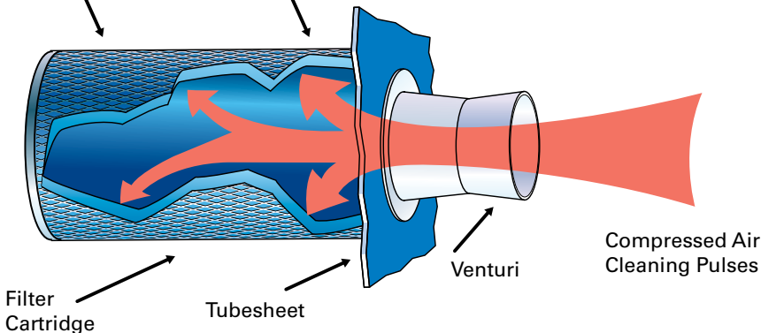
DOWNFLO PULSE PRESSURE GRADIENTS
